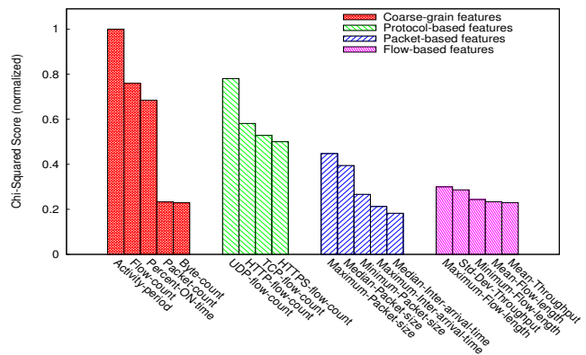
Fig. 5: Chi-Square statistic score for the highest-correlated features for each subset of statistical attributes.
